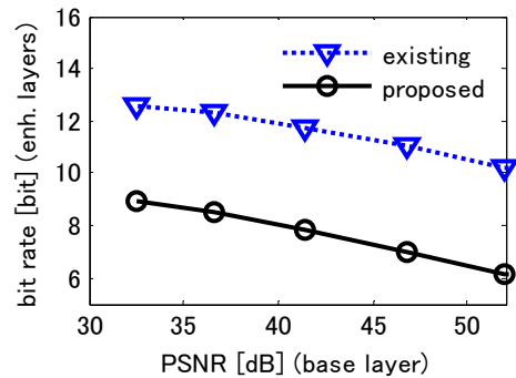
Fig.11 Bit rate of the enhancement layer (Luminance).
