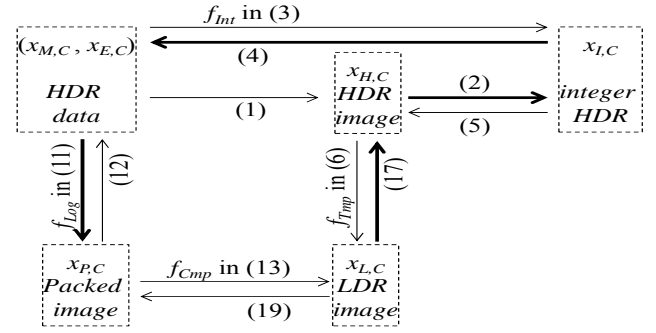
Fig.4 Relations among the mapping functions
