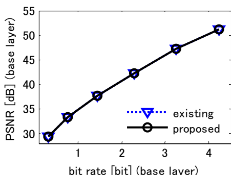
Fig.13 Rate distortion curves of the base layer (color).
