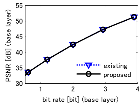
Fig.6 Rate distortion curves of the base layer (color).
