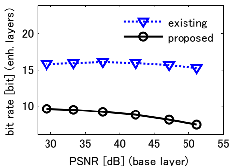
Fig.15 Bit rate of the enhancement layer (color).
