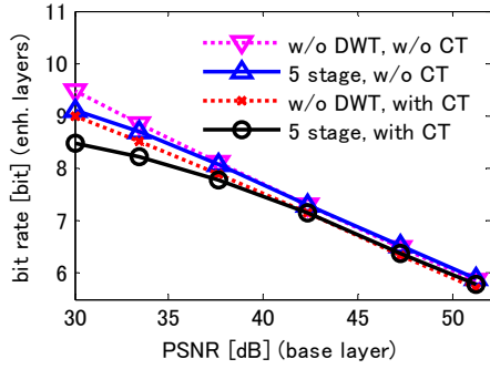
Fig.7 Bit rate of the enhancement layer (color).
