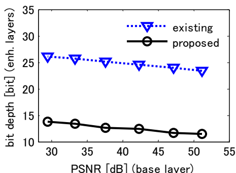
Fig.14 Bit depth of the enhancement layer (color).
