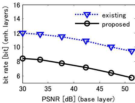
Fig.9 Bit rate of the enhancement layer (color).
