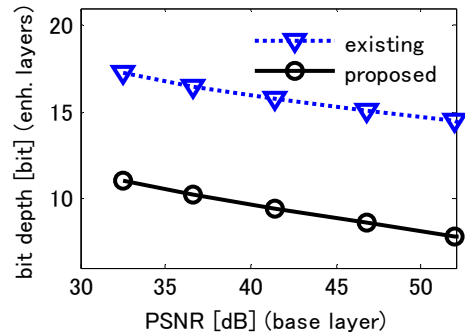
Fig.10 Bit depth of the enhancement layer (Luminance).
